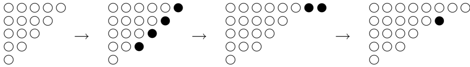
FIGURE 1. Insertion of \mu = (4, 2, 1) into \tau = (5, 4, 3, 2, 1) .
