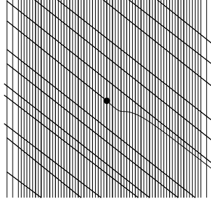
Figure 1: Closing up to a simple closed curve through z_1 .
