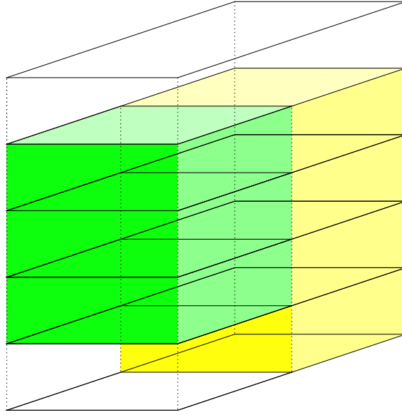
Figure 5: The figure shows two prisms (green and yellow) in M_\phi . The prisms stop near the top of the picture as the rectangles at the tops of the prisms are mixed: they are both mapped by \phi into the topmost rectangle in the picture. At the bottom of the picture, both rectangles are unmixed, but only one of the boxes (the yellow one) is filled. This means that the rectangle directly below the green prism is not Y -equivalent to its image by \phi , the bottom of the green prism (although it is h -equivalent).
