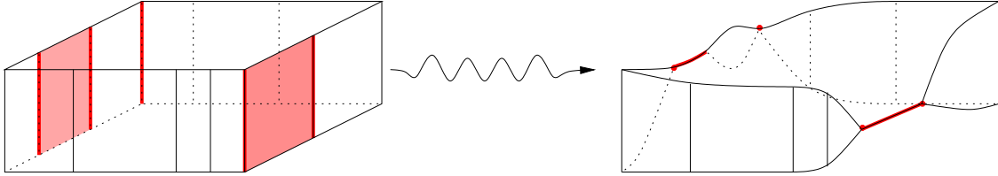
Figure 6: On the left is a box in M with the suspension cells contained in L shown in red. On the right is a picture of the 3-cell after collapsing the suspension cells of the boundary contained in L .
