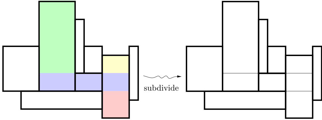
Figure 3: The image of the mixed rectangles are colored (see Figure 2) and they determine the subdivision of the original rectangles into subrectangles.
