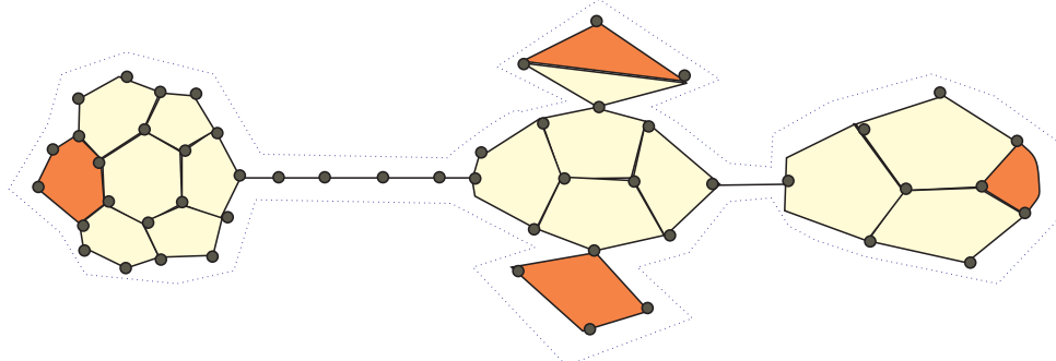
FIGURE 1. Illustrated above is a singular disc-diagram. The dotted path around the disc-diagram is meant to suggest the route of the boundary cycle of the disc-diagram. The shaded 2-cells in the diagram are complements of \leq 3 pieces. At least two such 2-cells are guaranteed by Greendlinger's Lemma.
