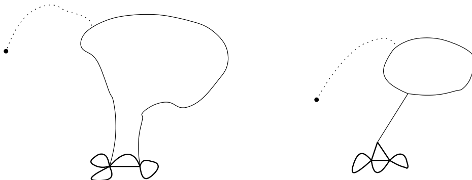
FIGURE 7. The two options for the graph \Delta
