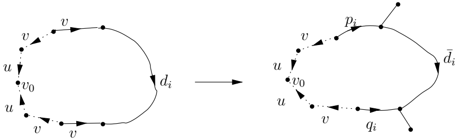
FIGURE 14. Constructing S_T^+ (only one loop drawn)
