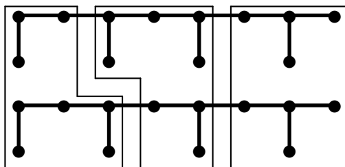
Figure 8: a_t(G_{4k} \square K_2) \leq 3
