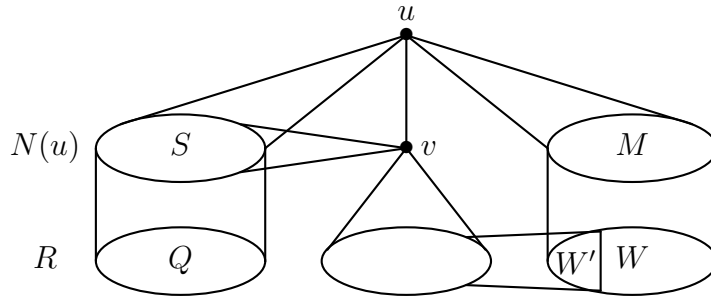
Figure 5: The structure of the diameter 2 graph G in Theorem 5.3.
