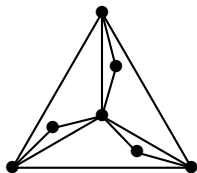
Figure 1: A non-3-colorable Eulerian plane graph
