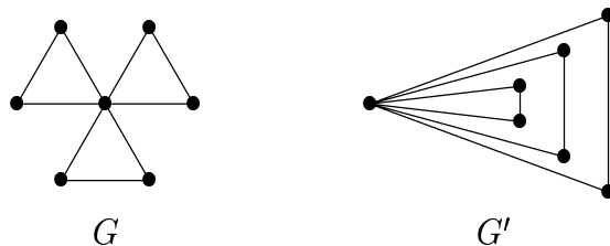
Fig. 1. Two embeddings of a planar graph.
