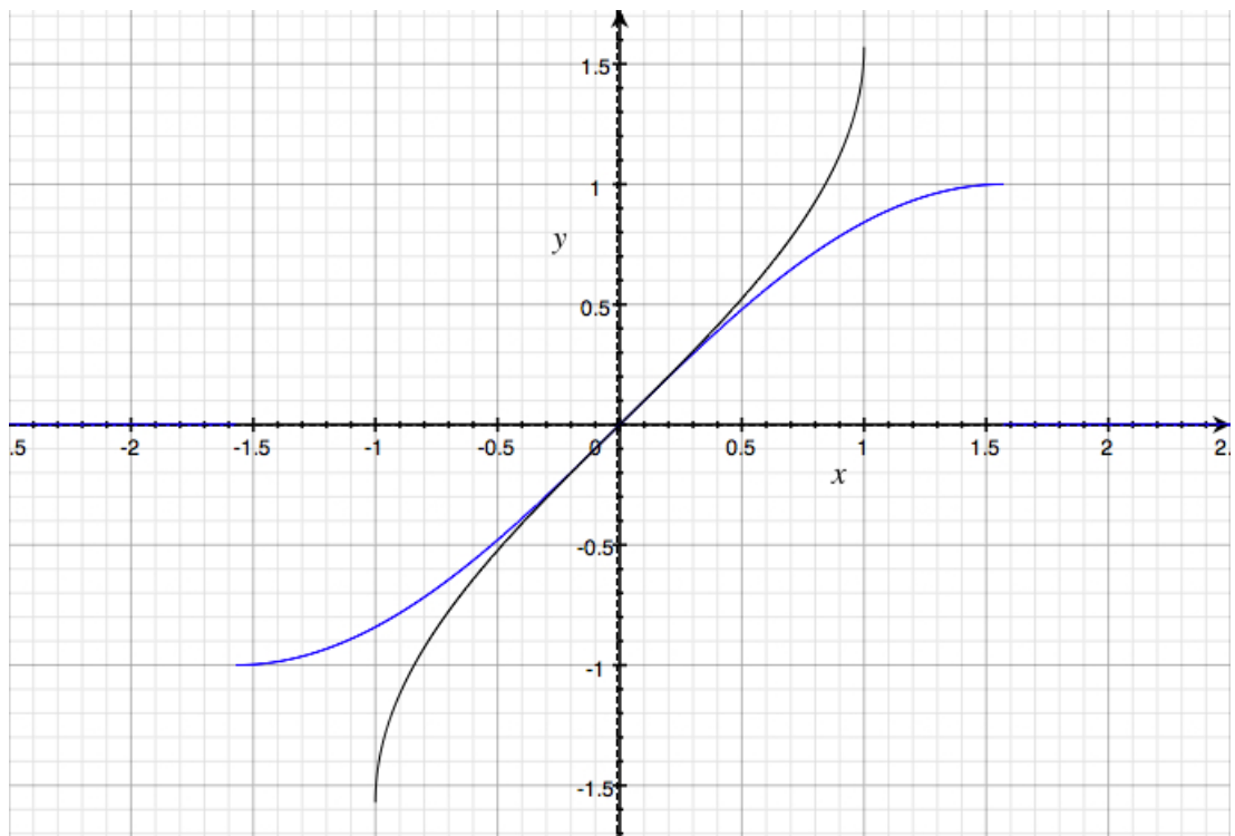
Figure 1: Sine is the blue curve, inverse sine is the black curve.
